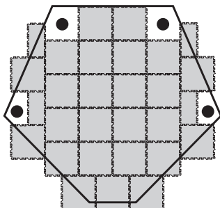
POTENTIAL LAYOUT IDEAS 660 / 980 SHELTER SIZES
